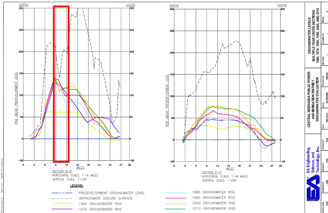
Figure 7 - Cross Section Near Proposed New E65 Canal Siphon
