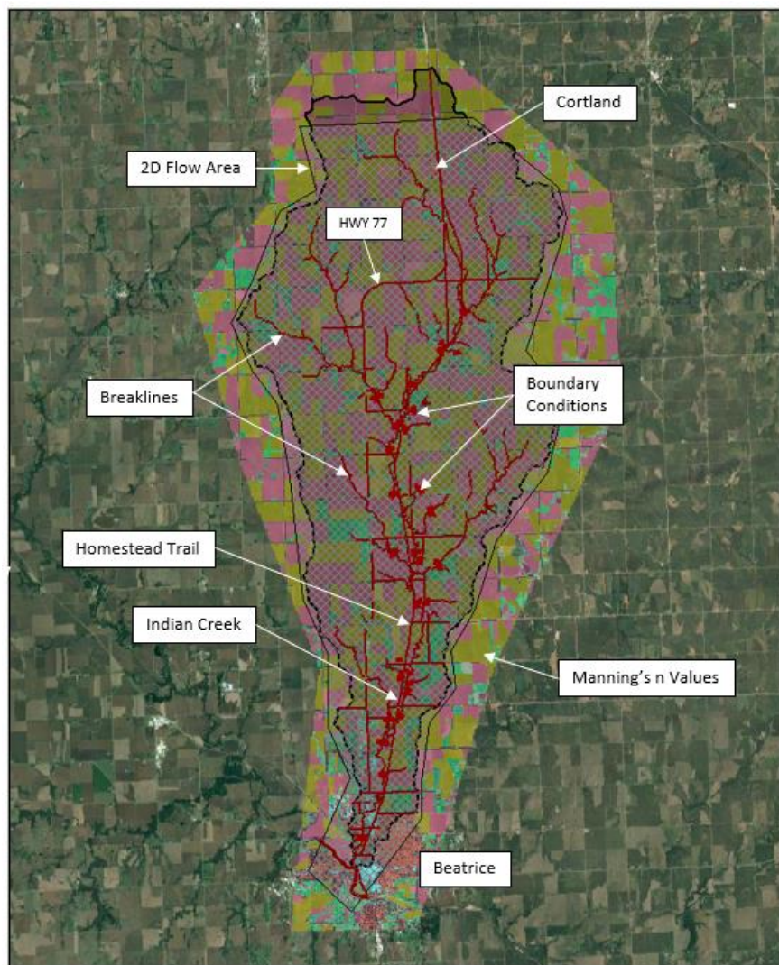
Little Indian Creek Hydraulic Model
