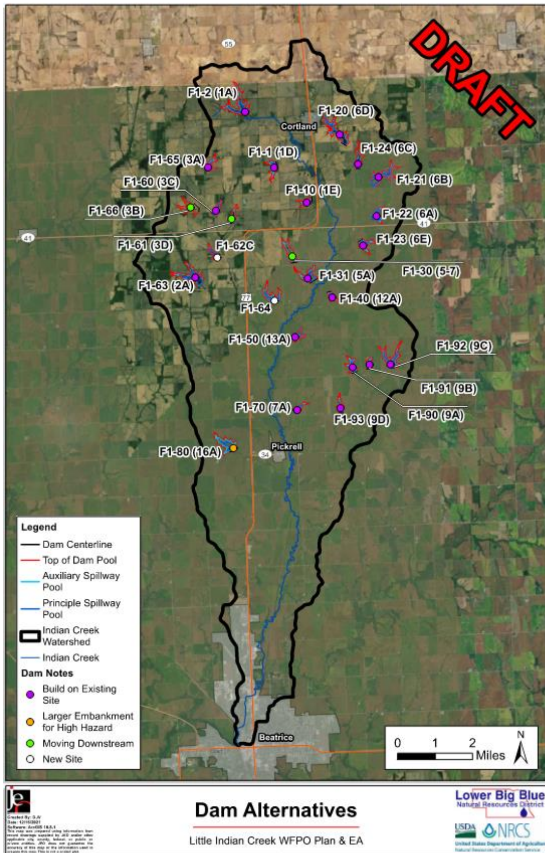
Map of planned structures in the Little Indian Creek Watershed.
